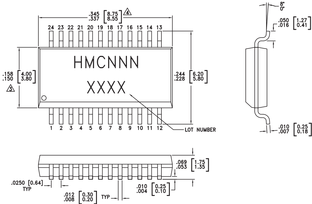
QS24 (E) Package Outline Drawing
